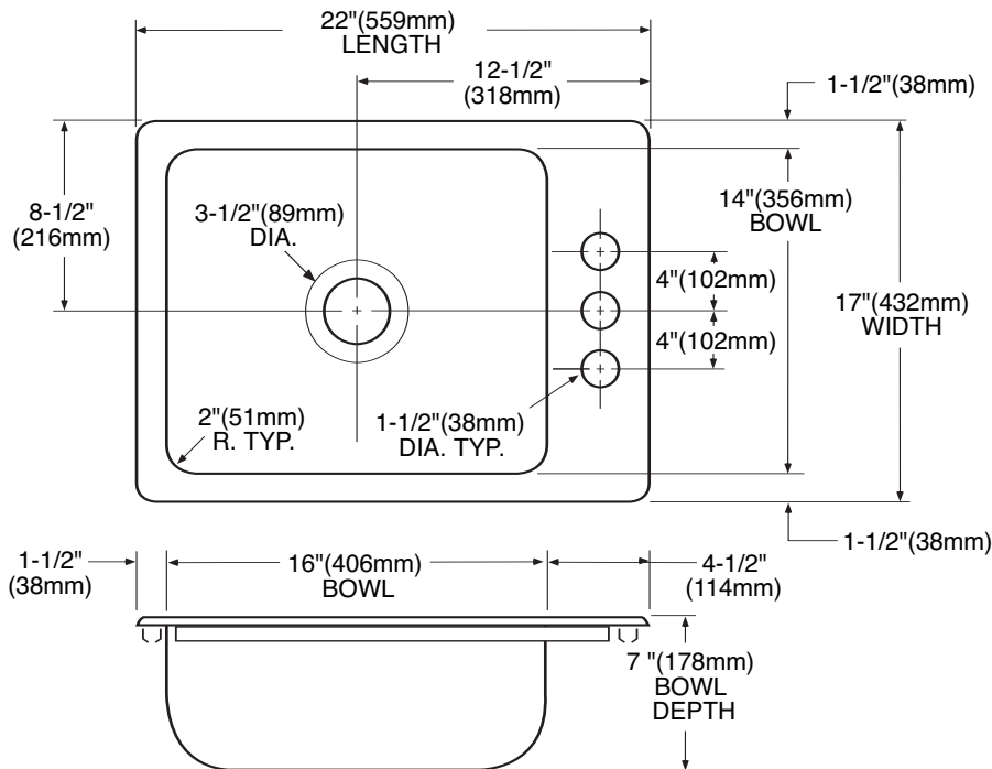
Installation Detail
