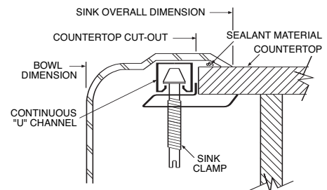
Installation Detail
