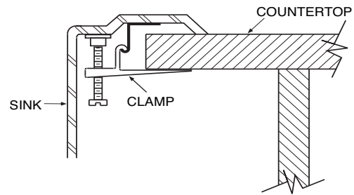
Installation Detail
